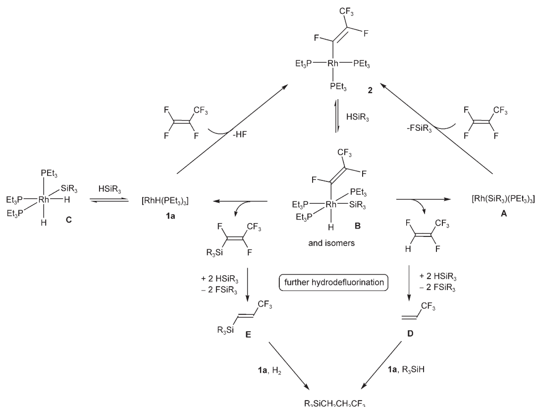
Scheme 3. Possible reaction pathways for the formation of (3,3,3-trifluoropropyl)silanes from hexafluoropropene.
