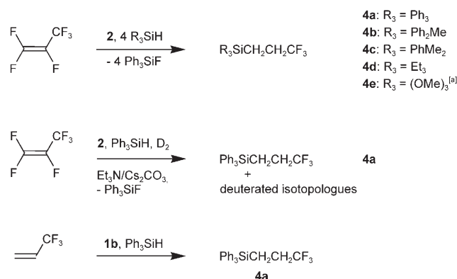
Scheme 2. Catalytic derivatization of fluorinated alkenes; [a] Et 3 N/Cs 2 CO 3 was added.
