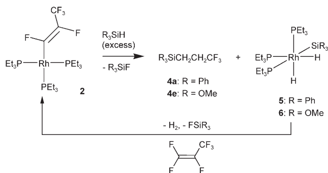
Scheme 1. Reactivity of 2 towards silanes.
